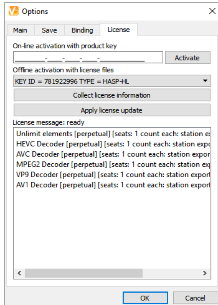
Figure 4. Creating a C2V file: License tab
