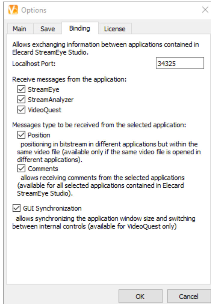
Figure 13. Elecard Video Quality Estimator GUI – Options – Binding Tab
