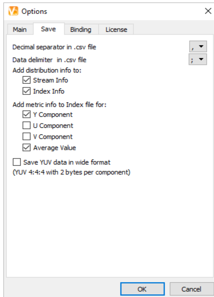
Figure 12. Elecard Video Quality Estimator GUI – Options – Save Tab
